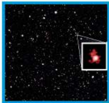
The furthest known galaxy, as seen by the Hubble space telescope, was probably formed about 400 million years after the Big Bang. It is shown here as it appeared 13.4 billion years ago.
