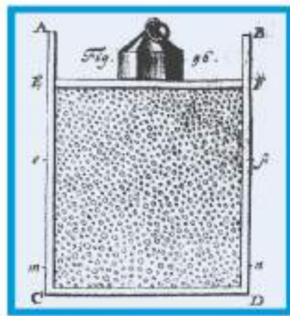
A diagram in Bernoulli's Hydrodynamica depicts air molecules colliding with the walls of a container, creating enough pressure to support a weight resting on a movable surface.
